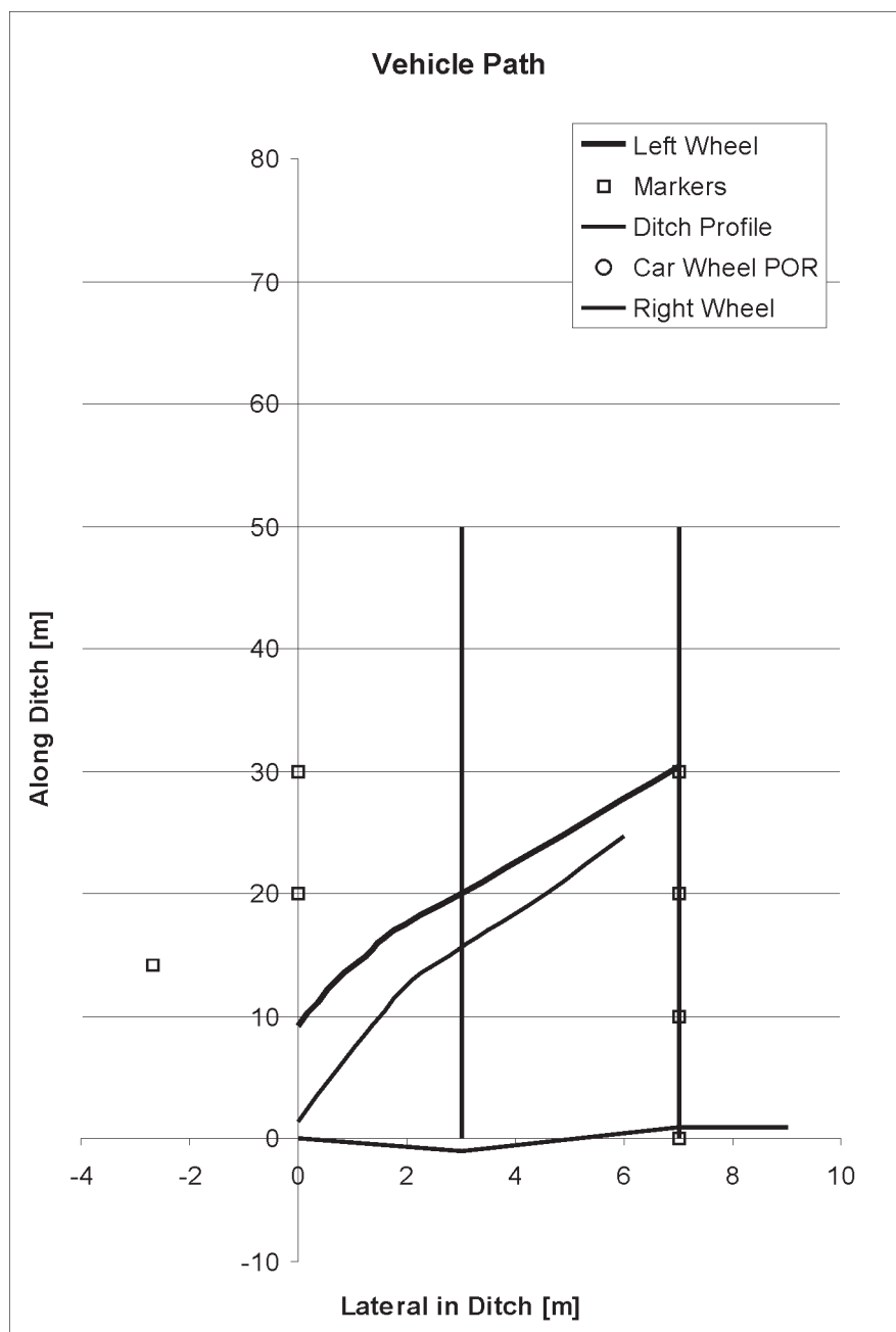
Test 15. Talbot Horizon, 96 km/h, 10,0 °
