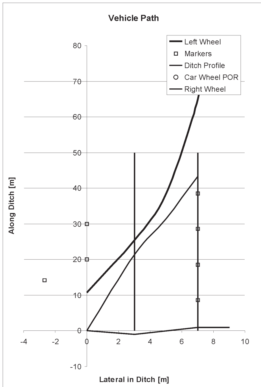
Test 1. Peugeot 205, 84 km/h, 4 °
