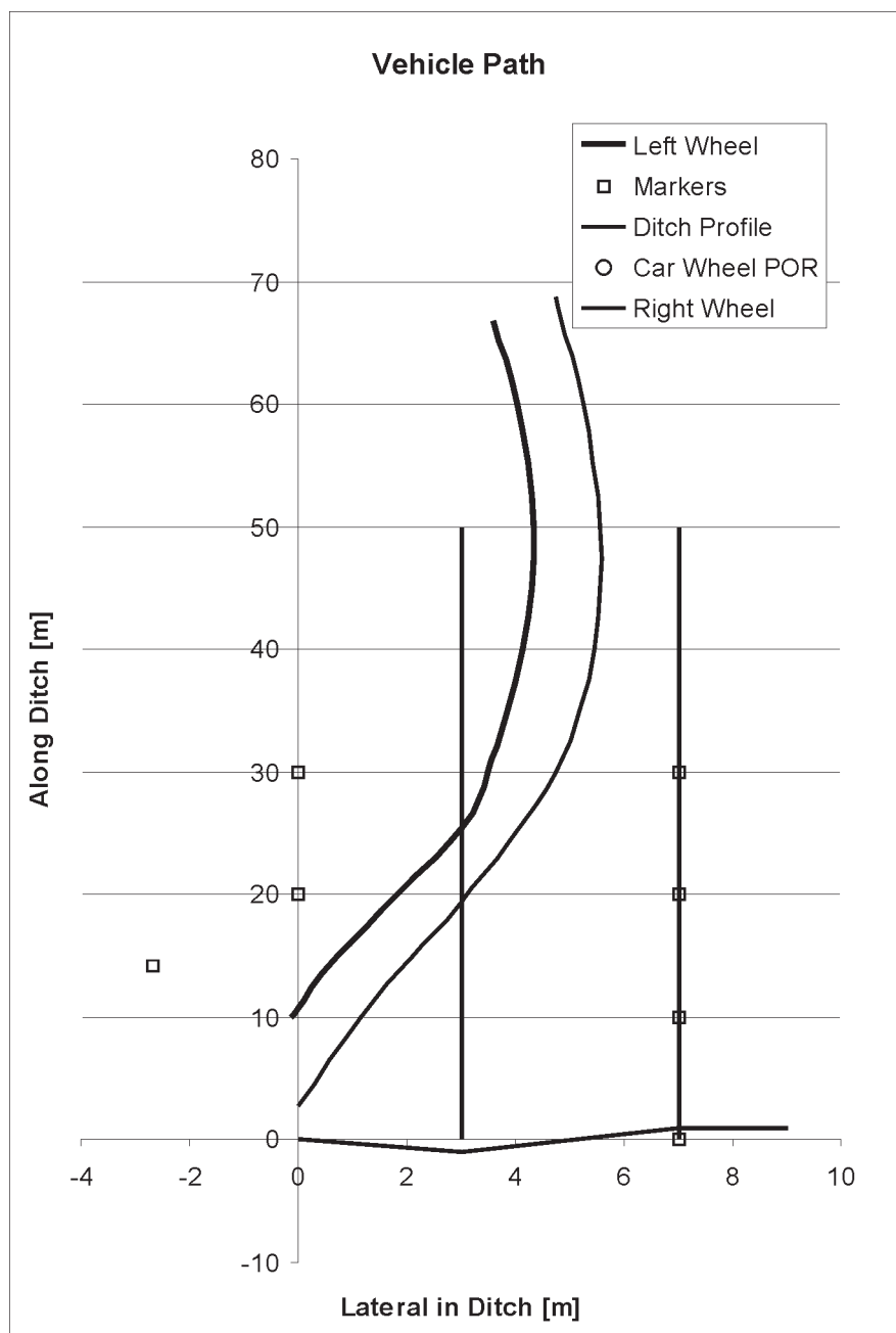
Test 13. Peugeot 205, 82 km/h 10,0 °
