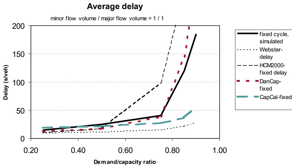
Figure F.1: Delays in pretimed intersection LIVASU with minor/major flow ratio 1
