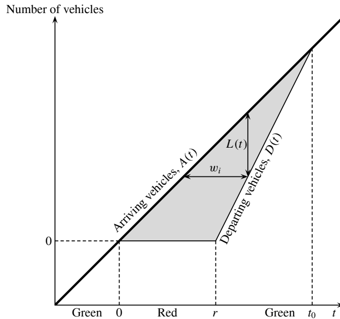
Figure 4.1: Fluid analogy model for traffic signal control
