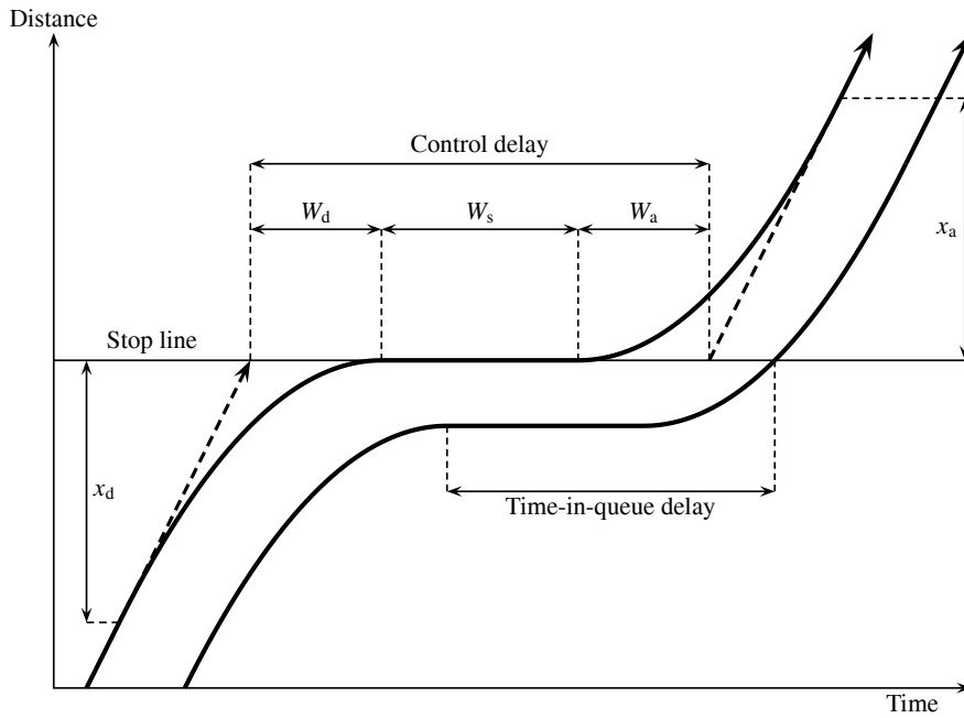
Figure 2.5: Delays at traffic signals
