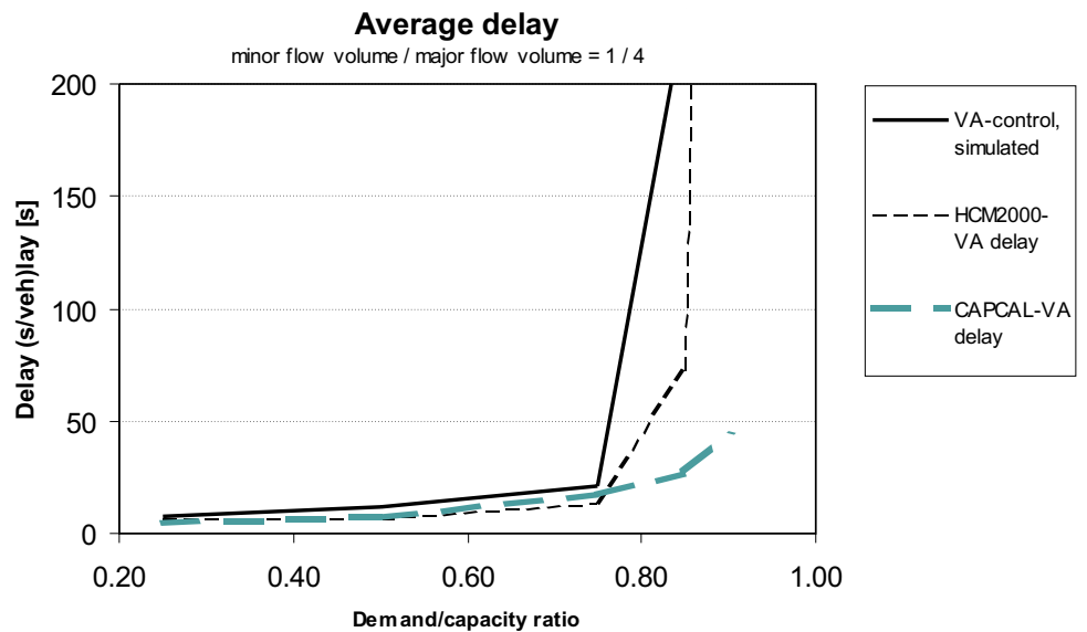
Figure E.14: Delays in traffic-responsive intersection HCM-2 with minor/major flow ratio 1/4
