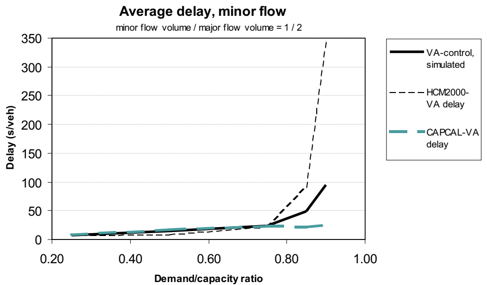
Figure B.12: Minor flow delays in traffic-responsive intersection Basic-2 with minor/major flow ratio 1/2 and 10% left turners
