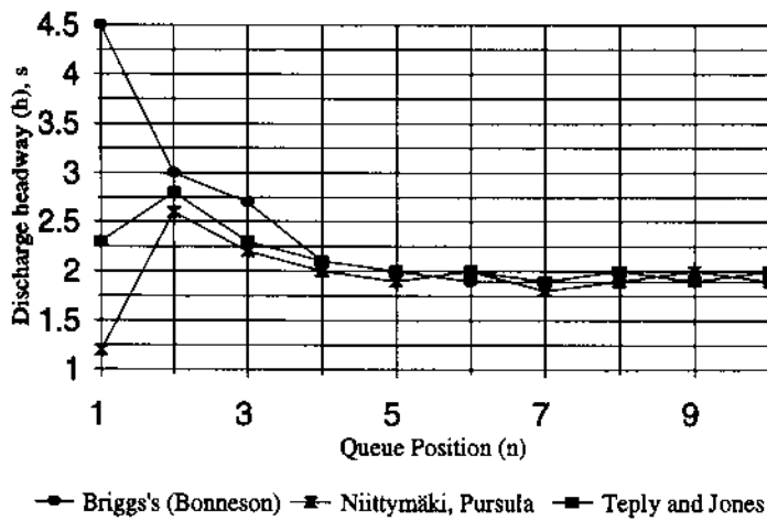
Figure 2.6: Discharge headways as a function of queue position (Niittymäki & Pursula 1997)
