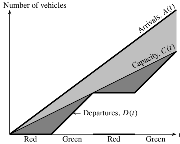
Figure 4.2: Fluid analogy model for overflow delay
