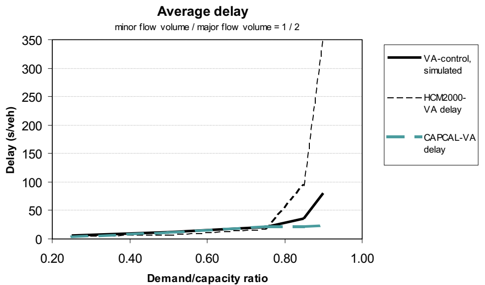
Figure B.8: Delays in traffic-responsive intersection Basic-2 with minor/major flow ratio 1/2 and 10% left turners
