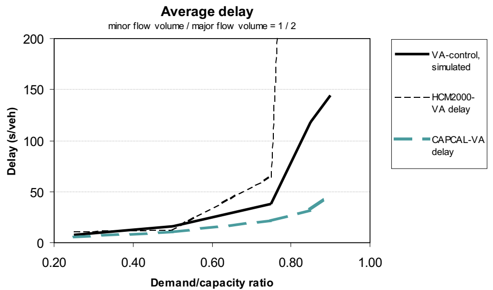
Figure F.8: Delays in traffic-responsive intersection LIVASU with minor/major flow ratio 1/2
