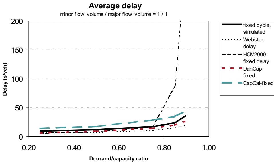
Figure D.1: Delays in pretimed intersection HCM-1 with minor/major flow ratio 1
