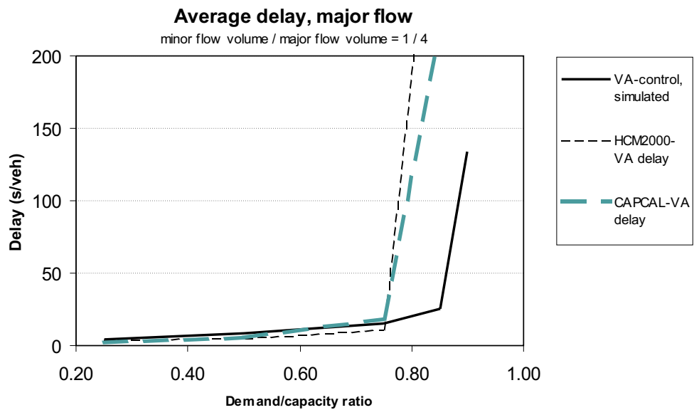
Figure D.16: Major flow delays in traffic-responsive intersection HCM-1 with minor/major flow ratio 1/4
