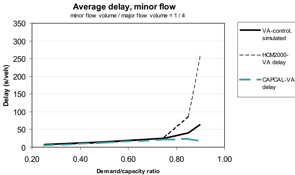
Figure B.18: Minor flow delays in traffic-responsive intersection Basic-2 with minor/major flow ratio 1/4 and 10% left turners
