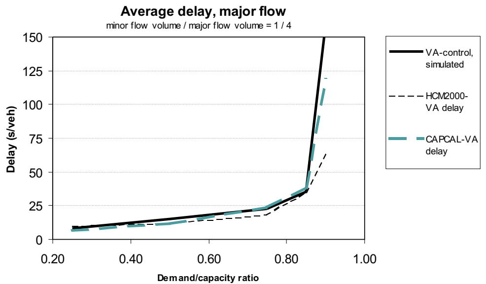
Figure F.16: Major flow delays in traffic-responsive intersection LIVASU with minor/major flow ratio 1/4
