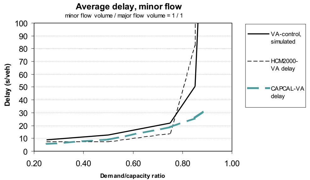
Figure E.6: Minor flow delays in traffic-responsive intersection HCM-2 with minor/major flow ratio 1
