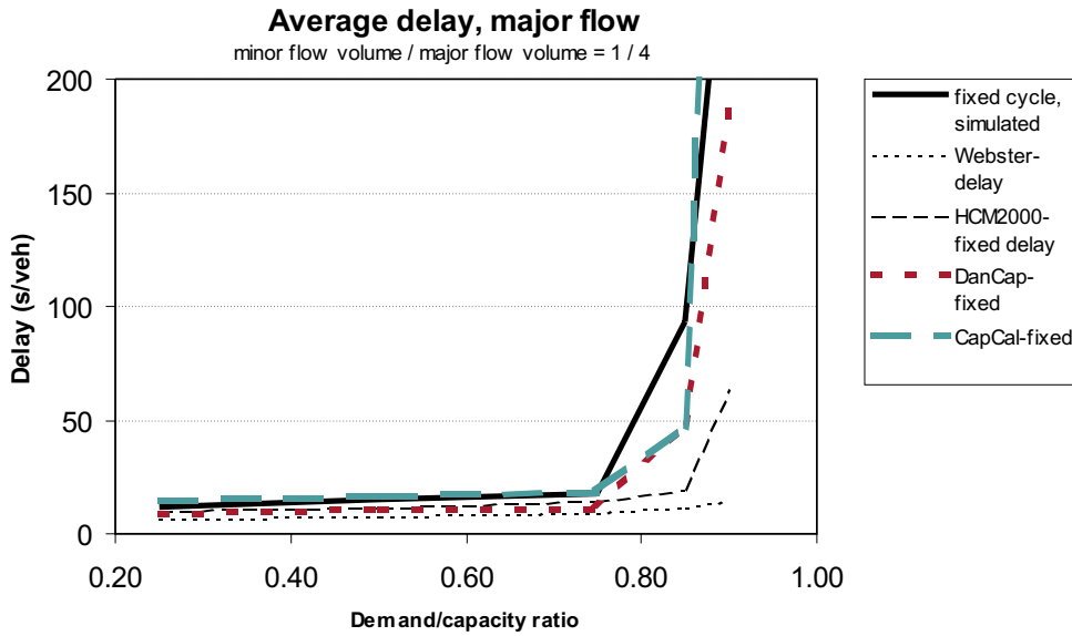
Figure E.15: Major flow delays in pretimed intersection HCM-2 with minor/major flow ratio 1/4
