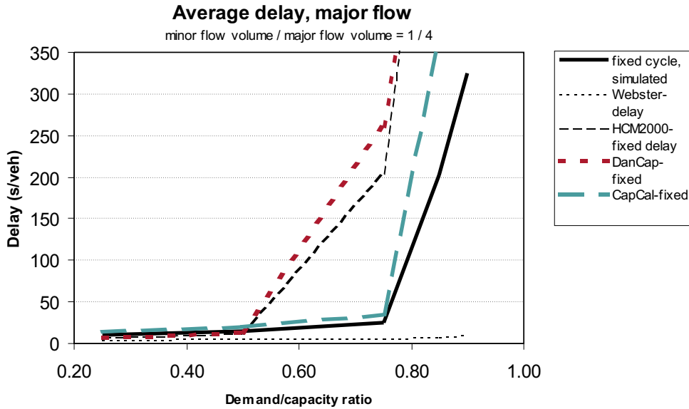
Figure C.15: Major flow delays in pretimed intersection Basic-2 with minor/major flow ratio 1/4 and 25 % left turners
