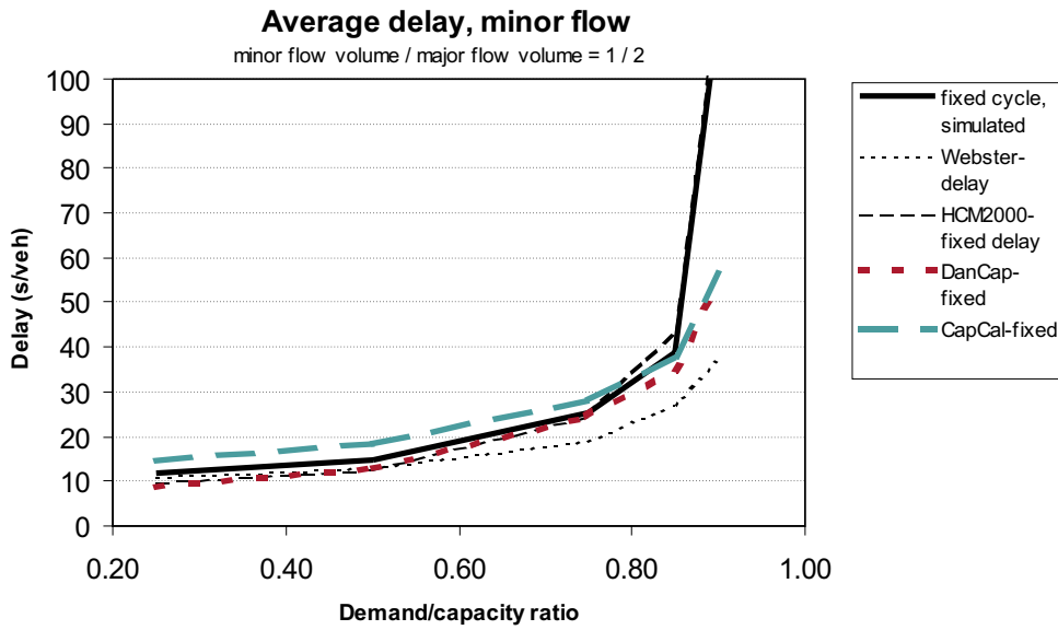
Figure E.11: Minor flow delays in pretimed intersection HCM-2 with minor/major flow ratio 1/2
