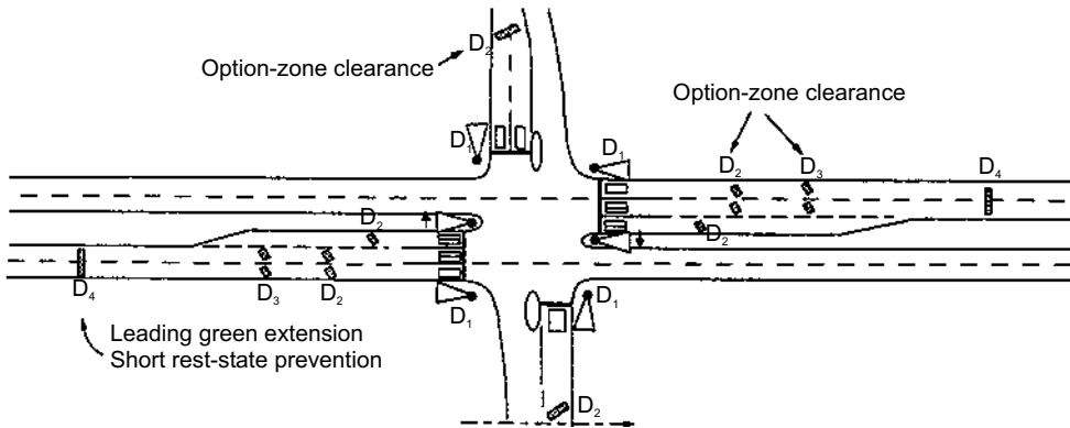
Figure 3.11: Detectors for the minimum functions. Adapted from Kehittämiskeskus (1996).
