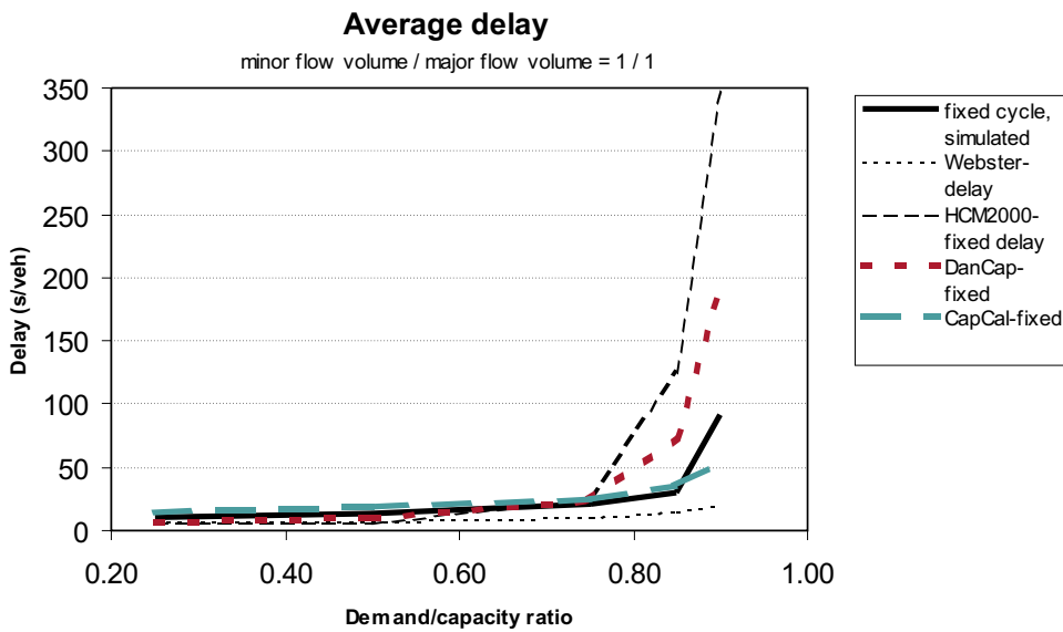
Figure B.1: Delays in pretimed intersection Basic-2 with minor/major flow ratio 1 and 10% left turners
