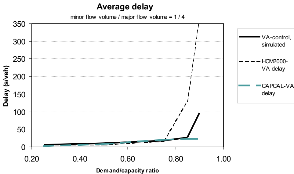
Figure B.14: Delays in traffic-responsive intersection Basic-2 with minor/major flow ratio 1/4 and 10% left turners
