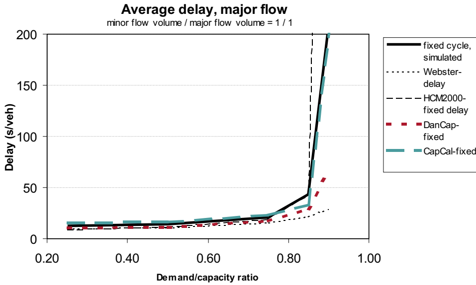
Figure E.3: Major flow delays in pretimed intersection HCM-2 with minor/major flow ratio 1
