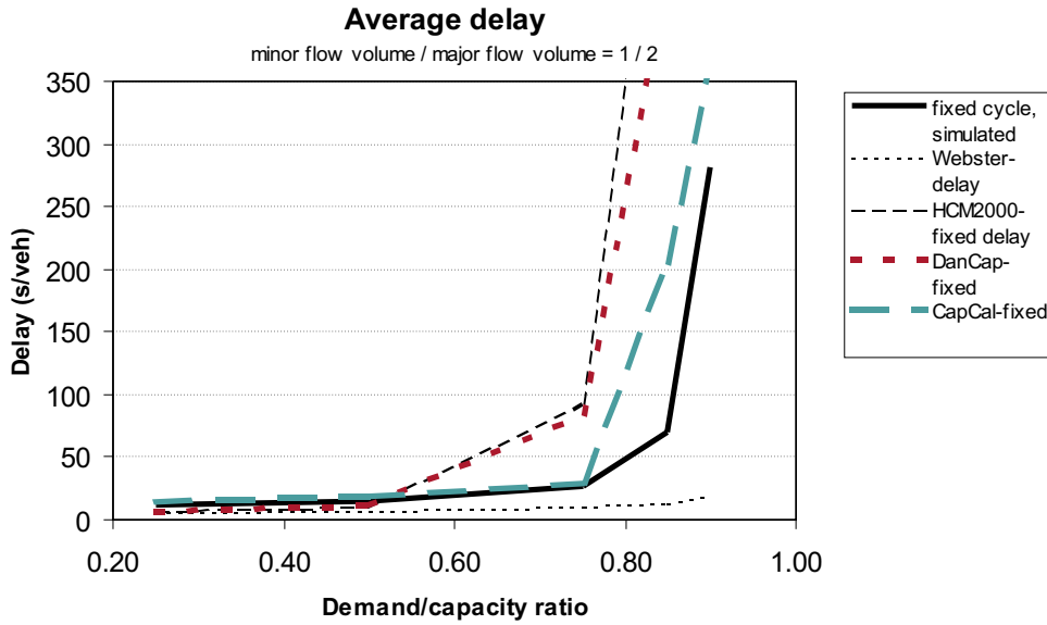
Figure C.7: Delays in pretimed intersection Basic-2 with minor/major flow ratio 1/2 and 25 % left turners
