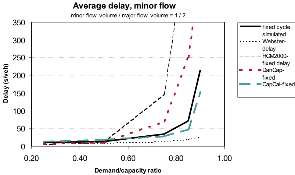
Figure C.11: Minor flow delays in pretimed intersection Basic-2 with minor/major flow ratio 1/2 and 25 % left turners
