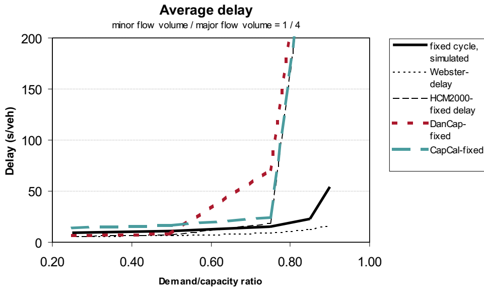
Figure D.13: Delays in pretimed intersection HCM-1 with minor/major flow ratio 1/4
