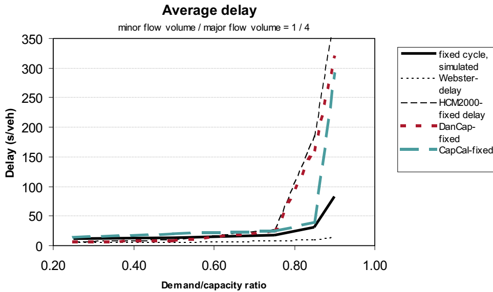
Figure B.13: Delays in pretimed intersection Basic-2 with minor/major flow ratio 1/4 and 10% left turners
