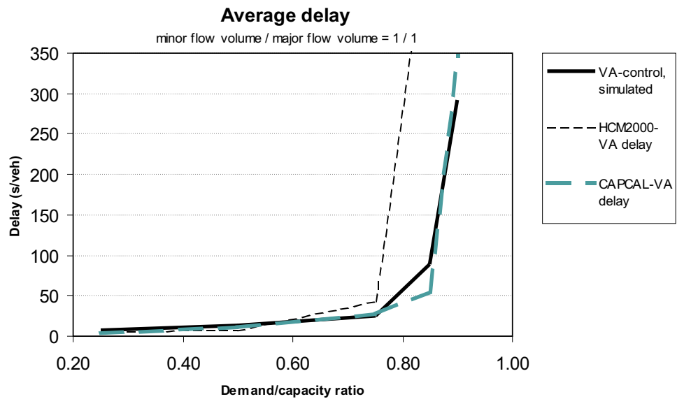
Figure C.2: Delays in traffic-responsive intersection Basic-2 with minor/major flow ratio 1 and 25% left turners
