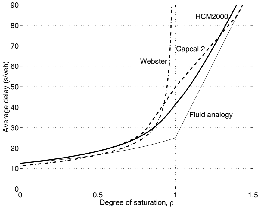
Figure 4.14: Delay in pretimed isolated intersections according to the fluid analogy model, shorter Webster equation (4.45), Capcal 2, and HCM2000 using the same parameters as in Figure 4.10
