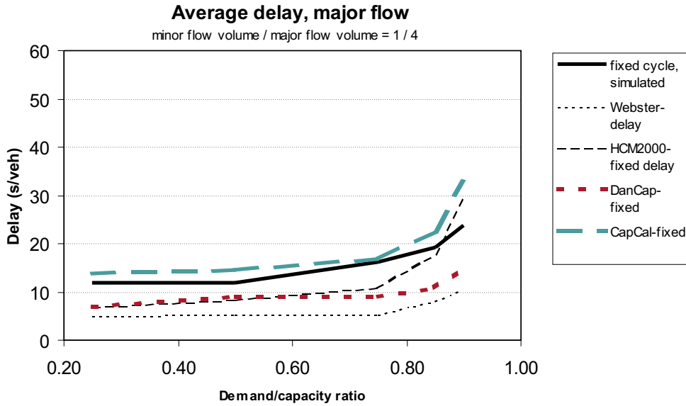
Figure A.15: Major flow delays in pretimed intersection Basic-1 with minor/major flow ratio 1/4
