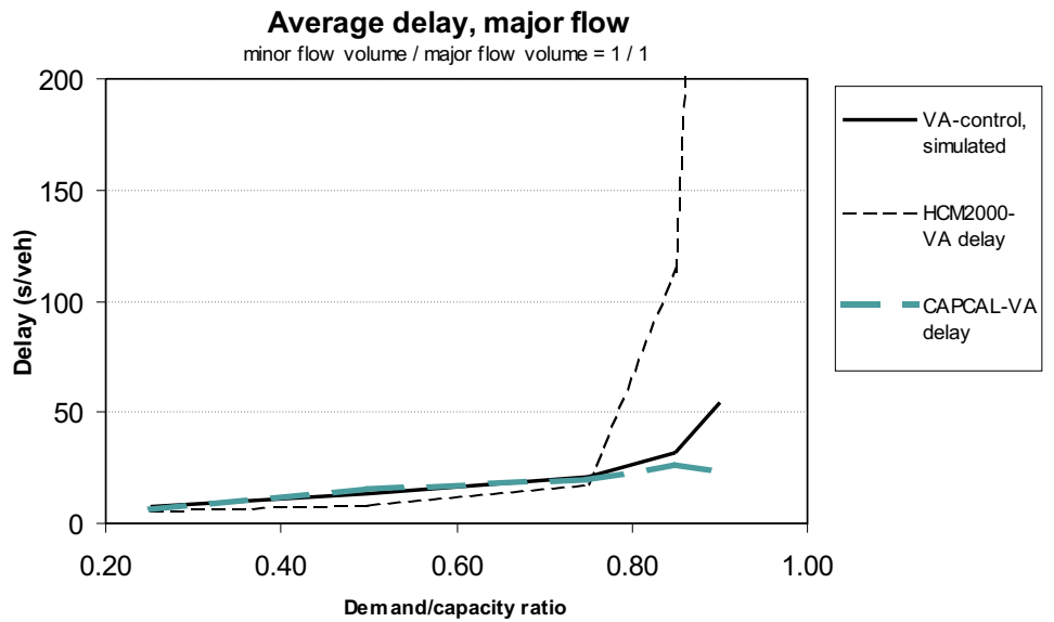
Figure D.4: Major flow delays in traffic-responsive intersection HCM-1 with minor/major flow ratio 1
