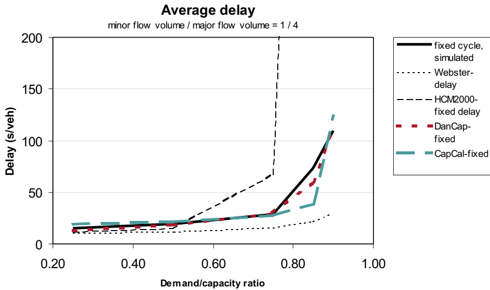
Figure F.13: Delays in pretimed intersection LIVASU with minor/major flow ratio 1/4
