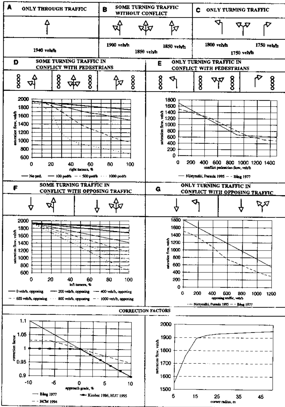
Figure 5.3: Finnish saturation flow guidelines (Niittymäki & Pursula 1997)
