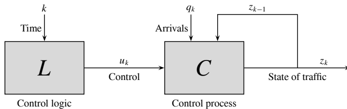
Figure 3.1: Pretimed traffic signal control process (Luttinen 1988)
