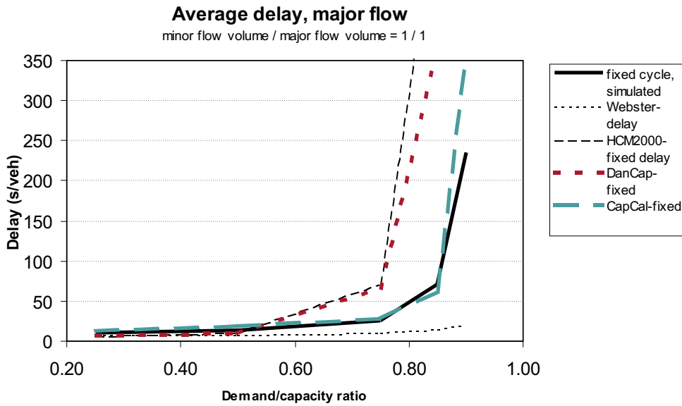
Figure C.3: Major flow delays in pretimed intersection Basic-2 with minor/major flow ratio 1 and 25 % left turners
