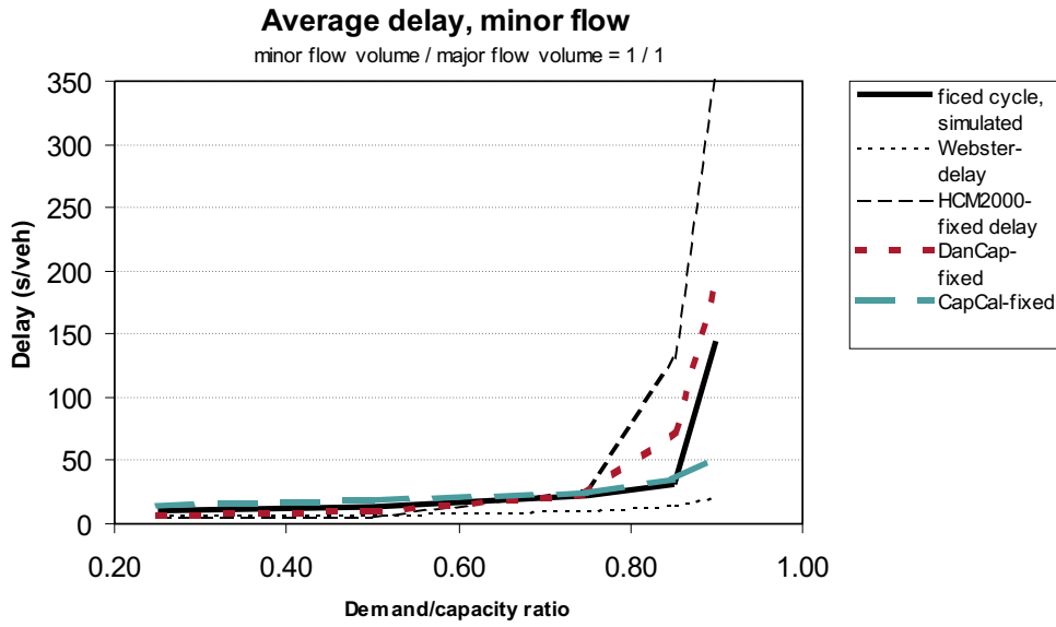
Figure B.5: Minor flow delays in pretimed intersection Basic-2 with minor/major flow ratio 1 and 10% left turners
