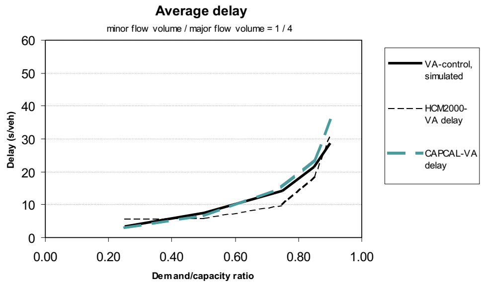
Figure A.14: Delays in traffic-responsive intersection Basic-1 with minor/major flow ratio 1/4
