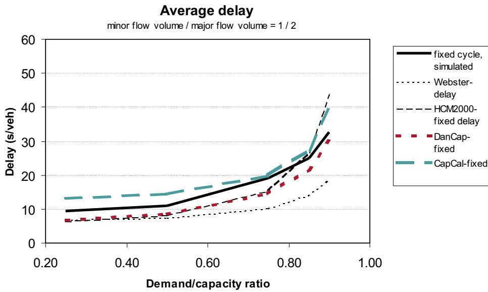
Figure A.7: Delays in pretimed intersection Basic-1 with minor/major flow ratio 1/2
