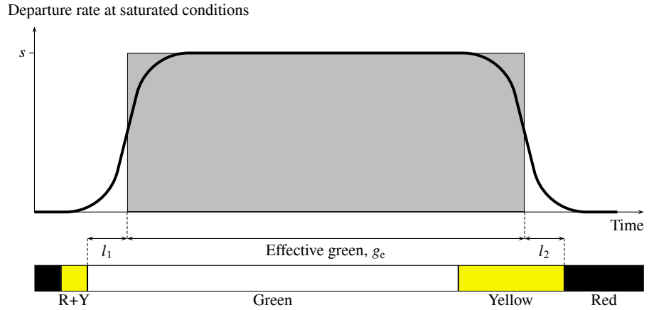
Figure 2.7: Departure rates and effective green
