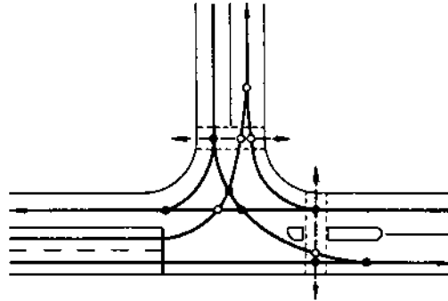
Figure 2.1: Primary (filled circles) and secondary (empty circles) conflict points in a T-intersection (Pohjoismaiden tietekillinen liitto 1978)
