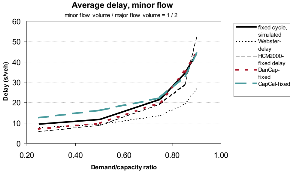
Figure A.11: Minor flow delays in pretimed intersection Basic-1 with minor/major flow ratio 1/2
