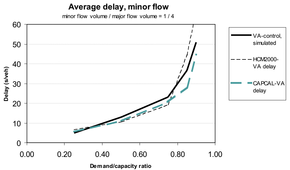
Figure A.18: Minor flow delays in traffic-responsive intersection Basic-1 with minor/major flow ratio 1/4
