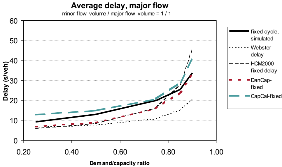
Figure A.3: Major flow delays in pretimed intersection Basic-1 with minor/major flow ratio 1
