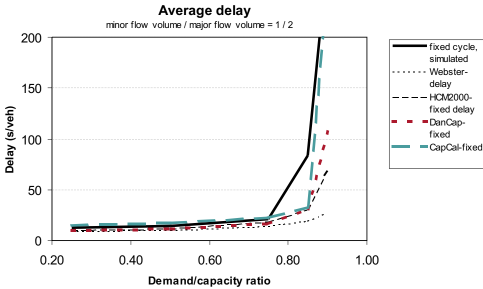
Figure E.7: Delays in pretimed intersection HCM-2 with minor/major flow ratio 1/2
