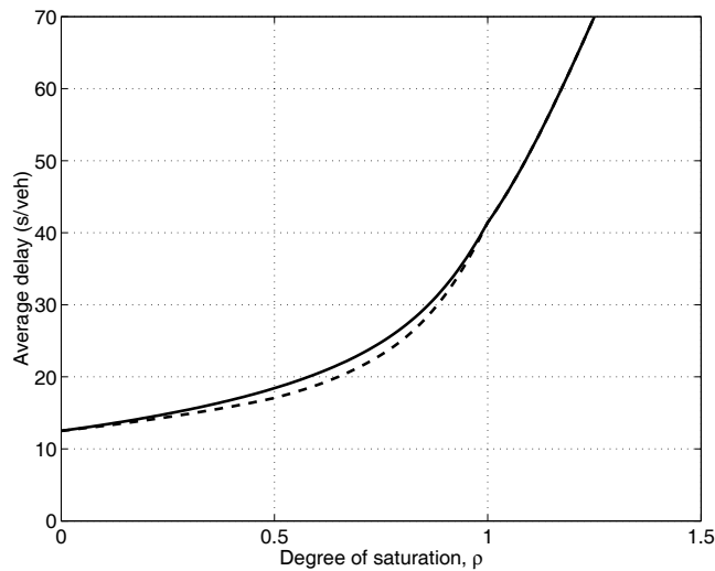
Figure 4.12: Delay in pretimed (solid curve) and traffic-actuated (dashed curve) isolated intersections according to HCM2000 using the same parameters as in Figure 4.10 and a three-second unit extension
