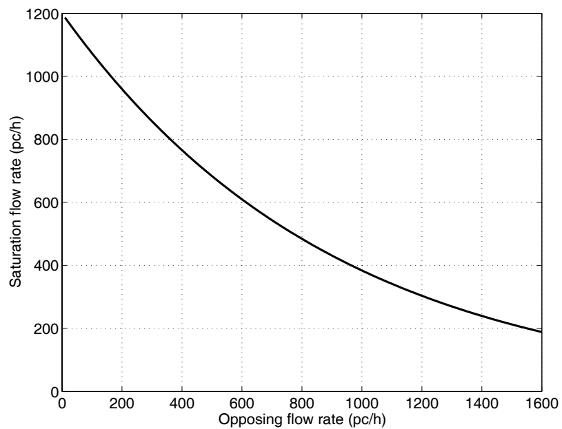
Figure 5.2: Basic saturation flow rate for permitted left turns according to DanKap (Vejdirektoratet 1999b)
