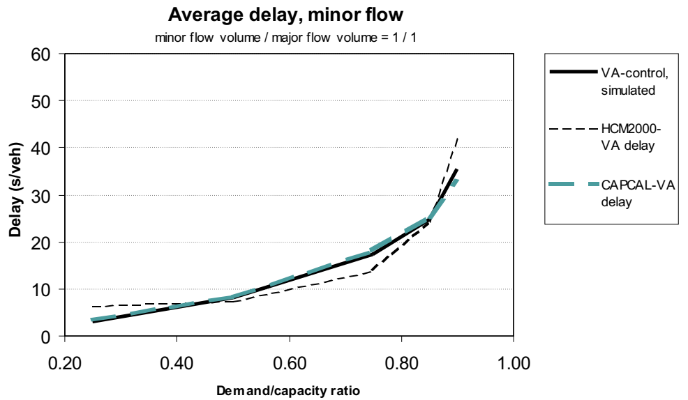
Figure A.6: Minor flow delays in traffic-responsive intersection Basic-1 with minor/major flow ratio 1
