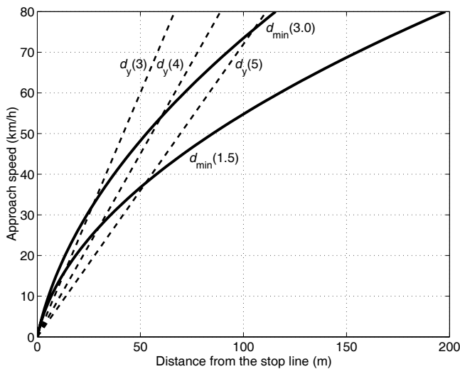
Figure 2.9: Maximum go-distances ( d_y , dashed lines) for yellow change intervals of 3, 4, and 5 s, and minimum stop-distances ( d_{min} , solid lines) for deceleration rates of 1.5 and 3.0 m/s^2
