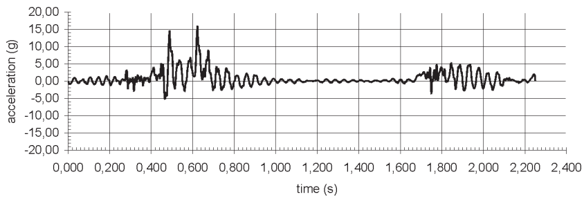
Y-acceleration
