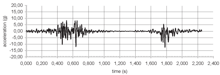
Z-acceleration
