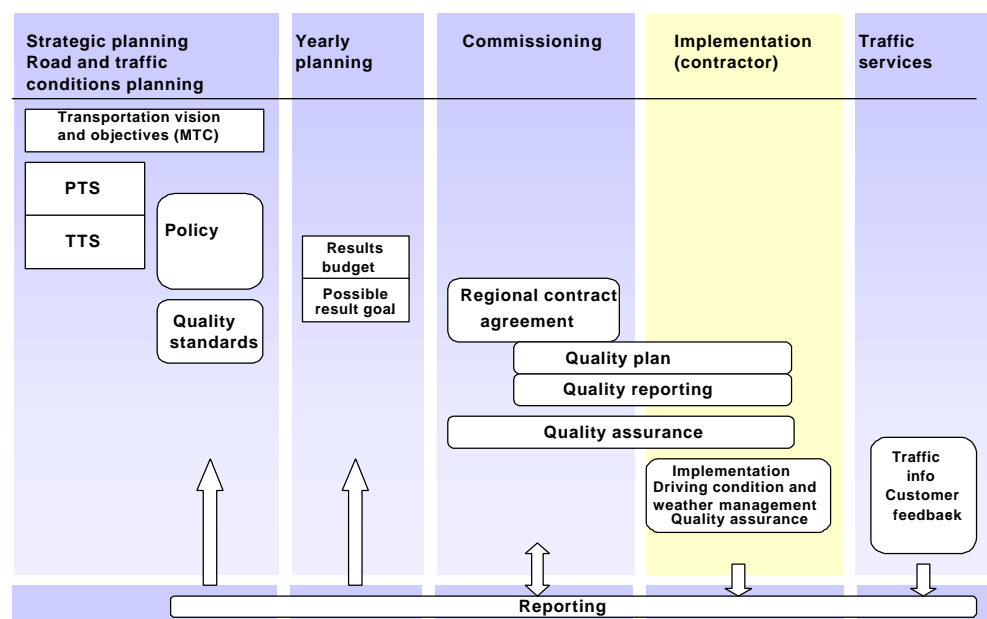
Figure 2. Phases of the control process of winter maintenance
