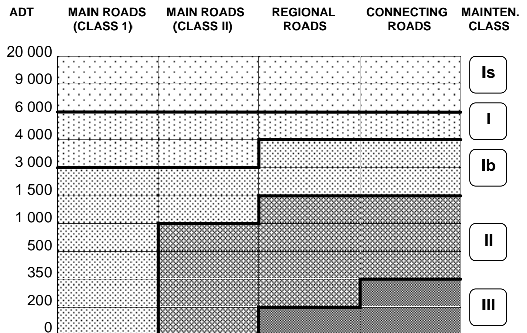
Figure 1. Division of the road network into winter maintenance classes.
