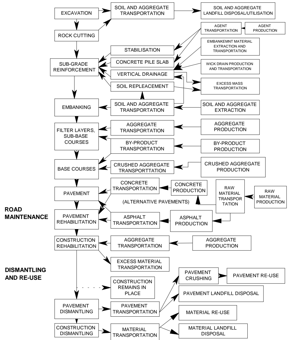
Figure 2. The principal road construction and usage phases which are taken into account when calculating environmental loadings of the structures.
