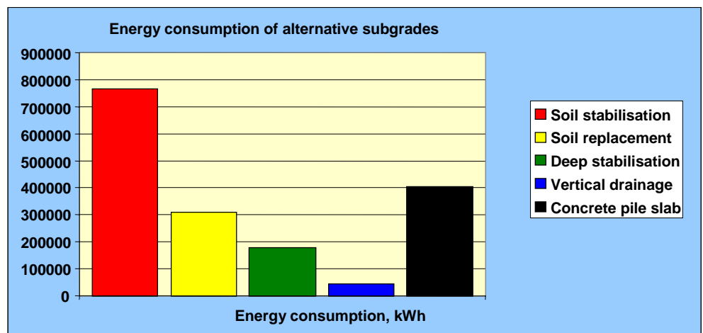
Figure 14. Fictive model presentation of the calculation program. Selected environmental loadings of alternative subgrades.
