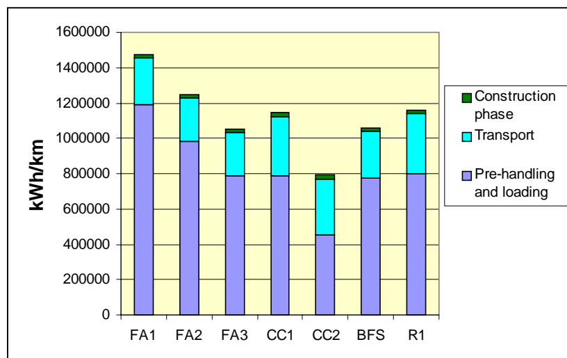
Figure 5. Energy consumption of the alternative structures.
