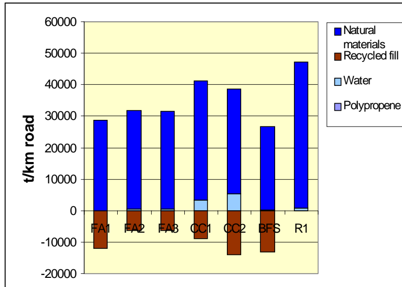
Figure 4. Consumption of raw materials in the pavement structures: FA1 – FA3 – fly ash constructions, CC1 and CC2 – crushed concrete constructions, BFS – blast furnace slag construction, R1 – natural aggregate construction.
