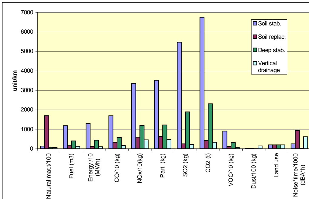
Figure 9. Environmental loadings of the alternative ground improvement and foundation engineering methods.
