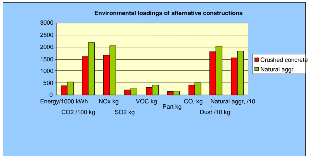
Figure 16. Environmental loadings of the alternative constructions of road case 1.
