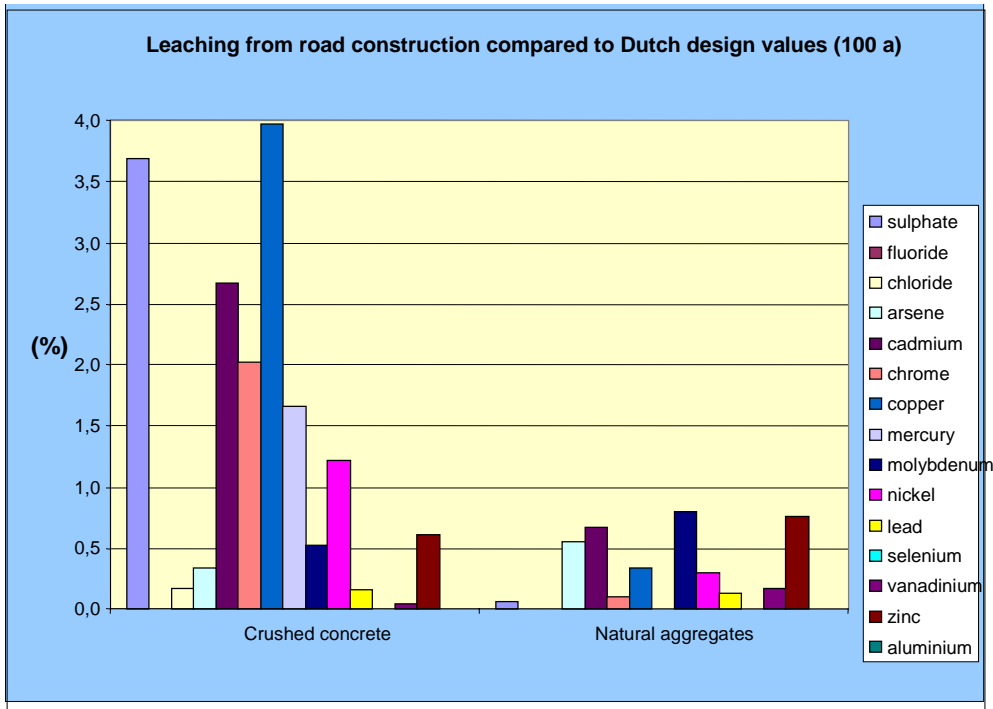
Figure 18. Impurities leaching out of the alternative constructions of road case 1 compared with the maximum permitted emission from materials/square metre over hundred years.
